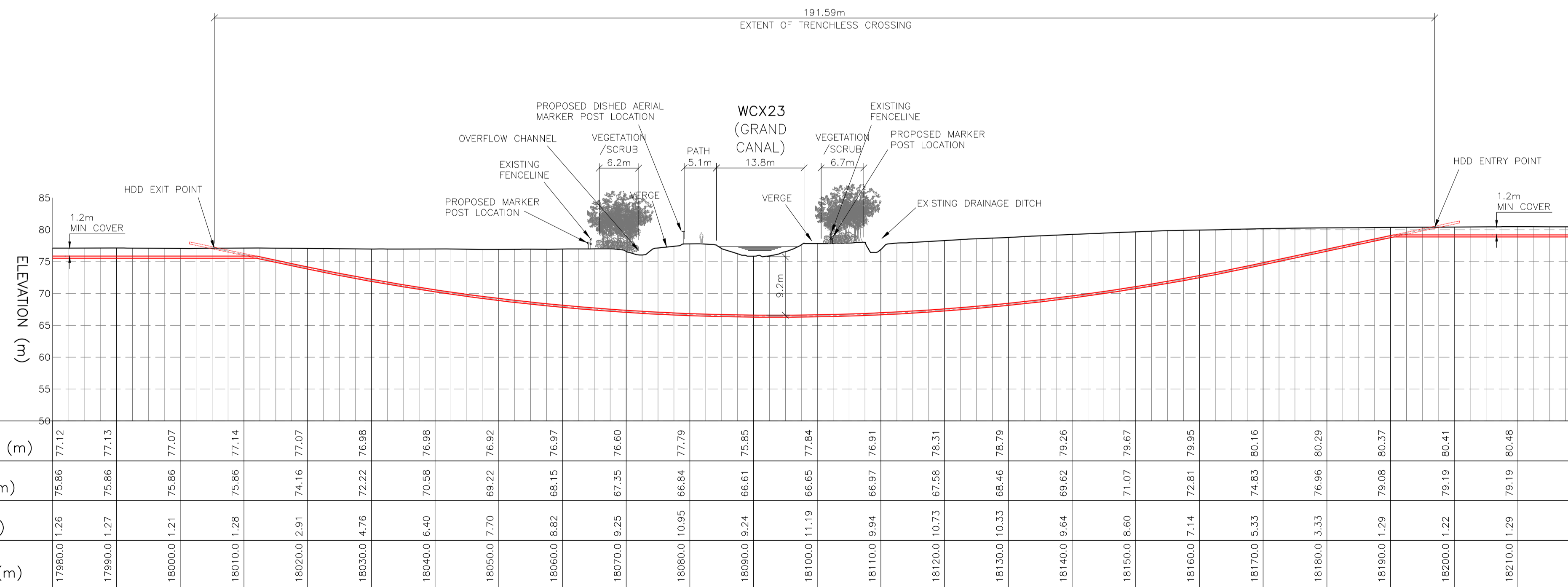
PROFILE ALONG PIPE CENTRELINE (SCALE 1:500)
